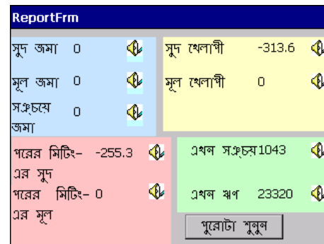
Fig. 6. Revised design of the RMTS-2 screen displaying updated payments, balances, and dues in color-coded quadrants
